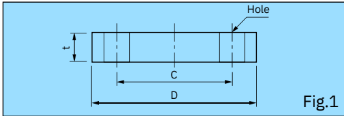
FLAT FACE (FF)
