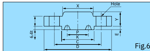
RING JOINT (RTJ)
