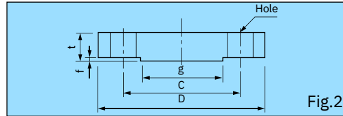
RAISED FACE (RF)
